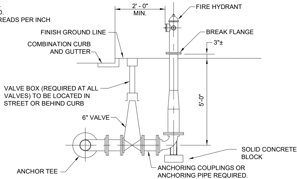
SECTION VIEW
