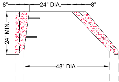
ECCENTRIC CONE TOP
