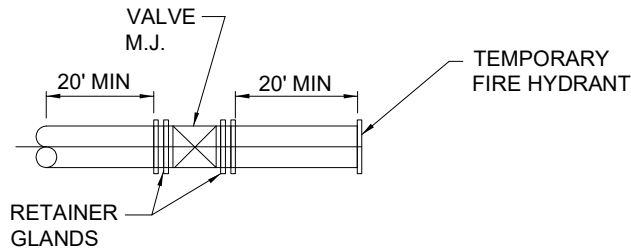
DETAIL - END OF WATER LINE
