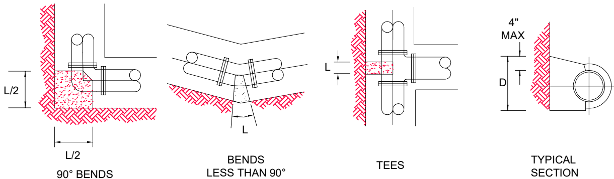
CONCRETE BLOCKING FOR HORIZONTAL BENDS
