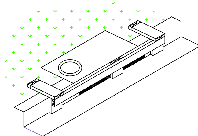
ISOMETRIC
