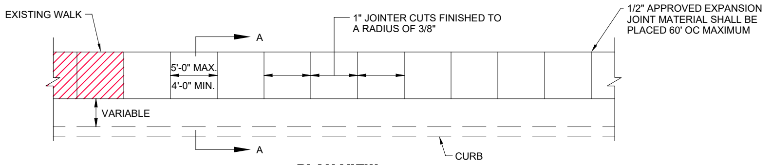
PLAN VIEW
