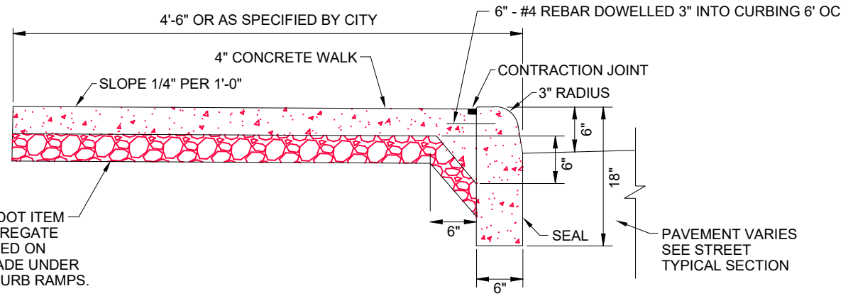
COMBINED CURB AND SIDEWALK DETAIL
