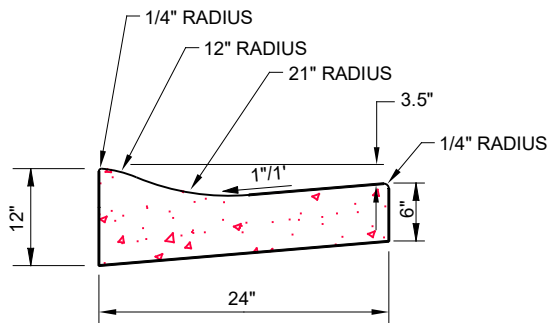
CITY OF PIQUA TYPE 1 CURB
