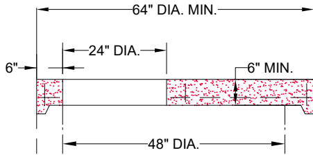
FLAT SLAB TOP
