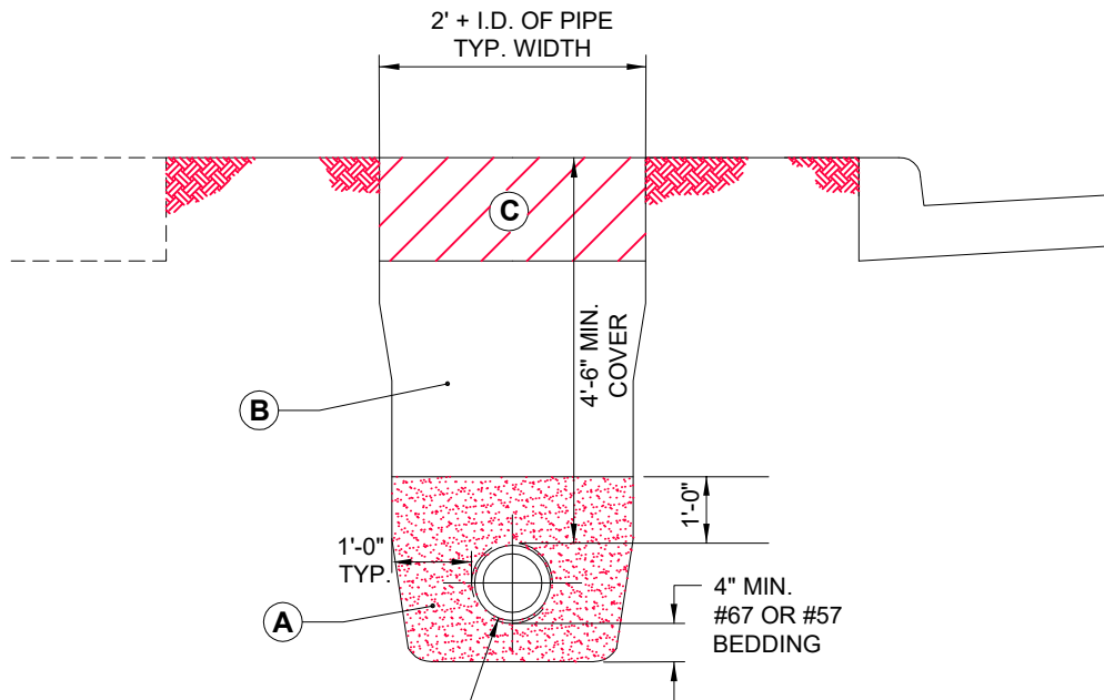
PROPOSED WATER MAIN WATER MAIN TRENCH DETAIL
