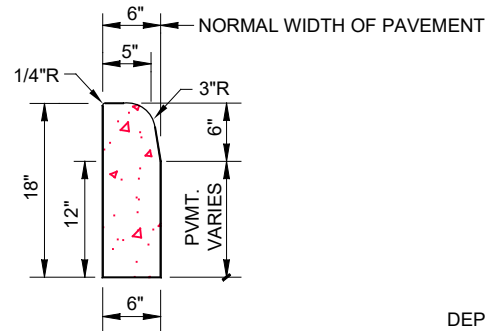
TYPE 6 BARRIER CURB
