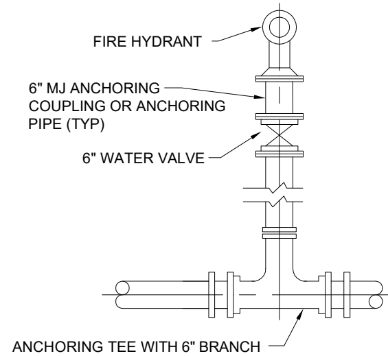
BASIC TEE DETAIL PLAN
