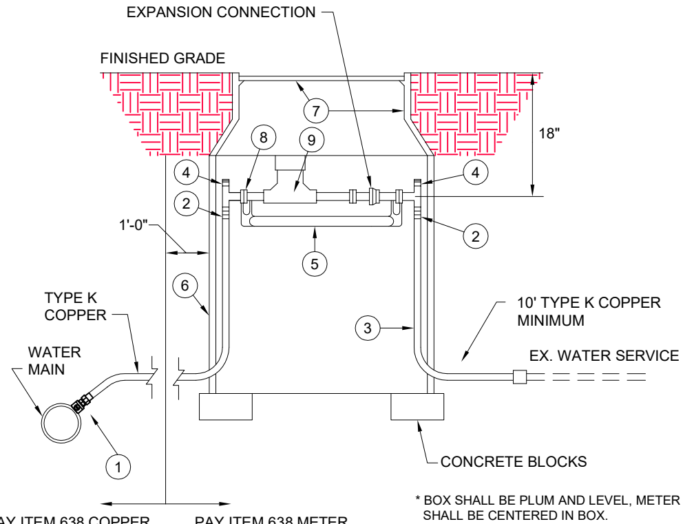
METER PIT DETAIL FOR 3/4" AND 1"
